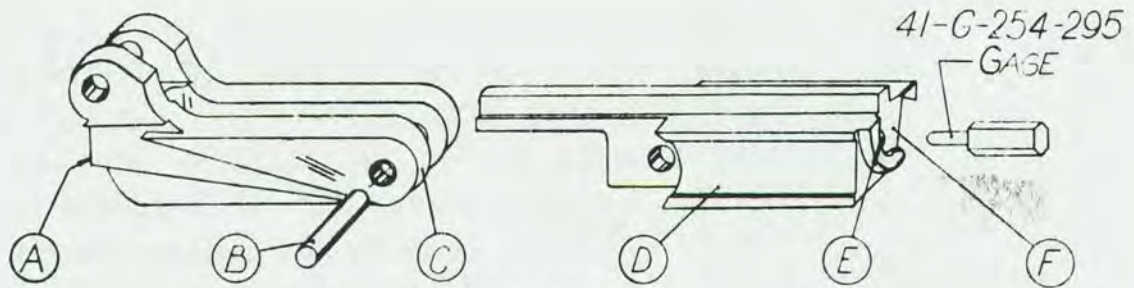
BOLT ASSEMBLY
