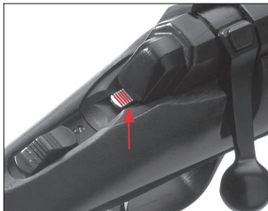
Location of the cocking indicator, shown in the cocked position.
