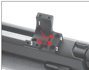
Tighten the screws incrementally in the pattern shown above.
