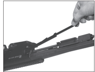
Pull the action bars forward and out of the receiver.
