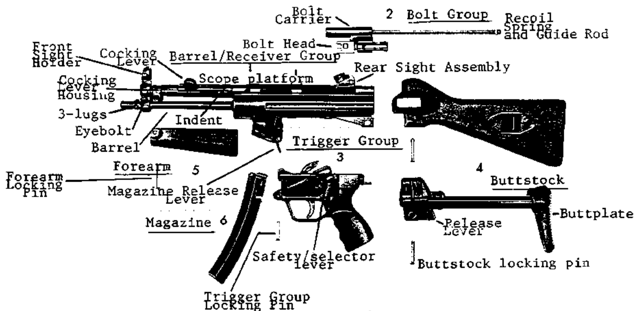
III.# 15A - Assembly Groups (MP5A2/A3 pictured)
