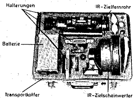
Transportkoffer
