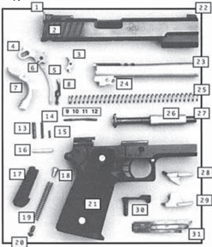
Typical Parts Breakdown - STI "1911/2011" Series
