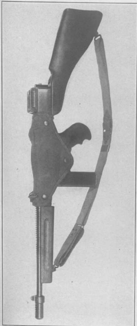
Thompson Gun breech cover for the protection of gun mechanism—can be instantly taken off by one continuous pull on cover flap. After being detached in an emergency, a leather thong holds cover on gun so it will not be lost.
