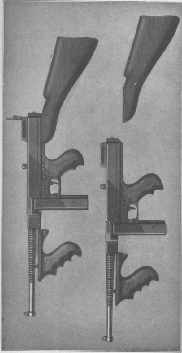
Thompson Gun calibre .45 with butt stock attached and sight leaf up; and gun with leaf down and butt stock removed.
