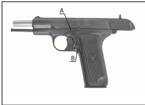
Fig. 2> Slide in rear position (A) – coupling, (B) – magazine release button
