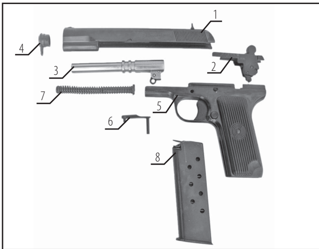
Fig. 13> Stripped pistol
