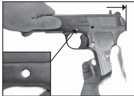
Fig. 15> Position of parts before inserting coupling
