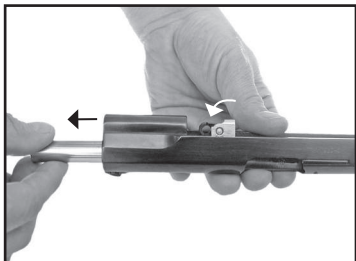
Fig. 12> Separating the barrel
