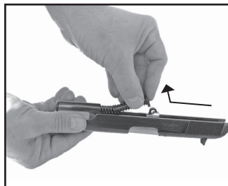
Fig. 10> Taking out the recoil mechanism (recoil spring with guide)
